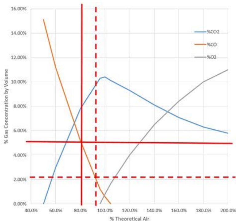
Figure I – Theoretical Combustion
