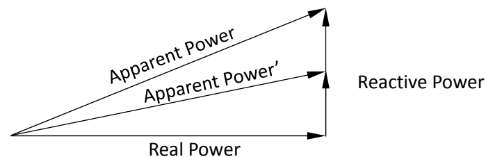
Figure 1: Power triangle for Apparent Power, Real Power and Reactive Power (Note: Apparent Power' refers to the apparent power after power factor correction)
